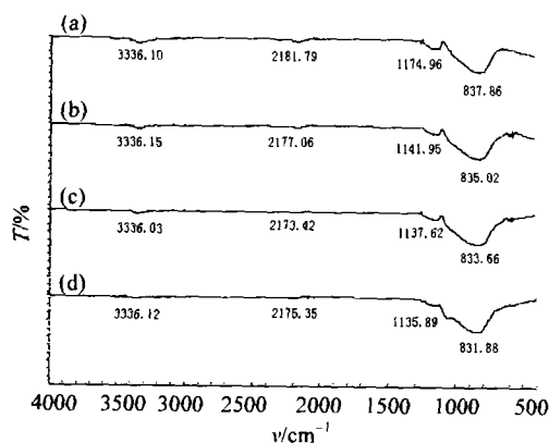
Fig. 2 IR absorption spectra for SiN films
